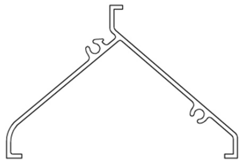
Figure 3 - ASK50 Chevron Louvre Blade.
