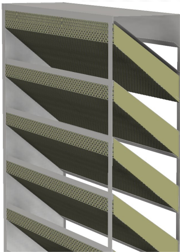
Figure 2 - Type WSD150 (150mm Deep) Single Bank Acoustic Louvre
